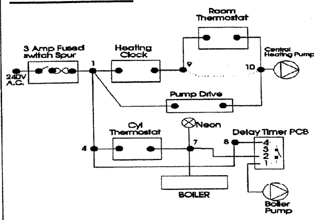
Figure 17 FLOW DIAGRAM
