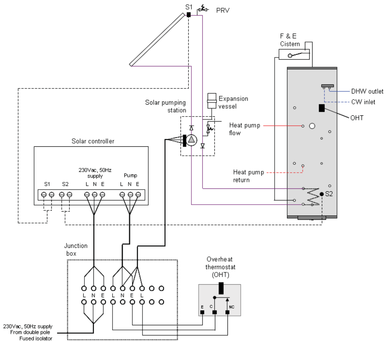
Typical schematic wiring diagram and system configuration for the Torrent GreenHeat HP-solar.
