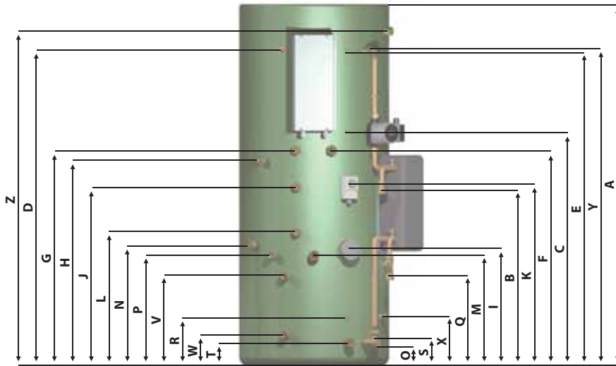
Torrent GreenHeat SOL
