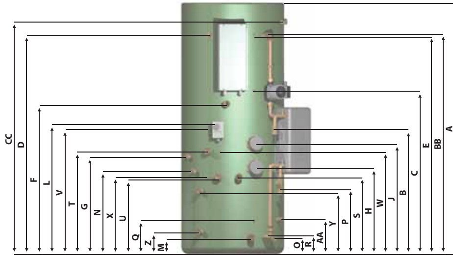
Torrent GreenHeat HP SOL
